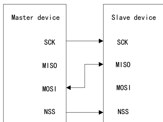
Figure 91 Bidirectional Line Connection
