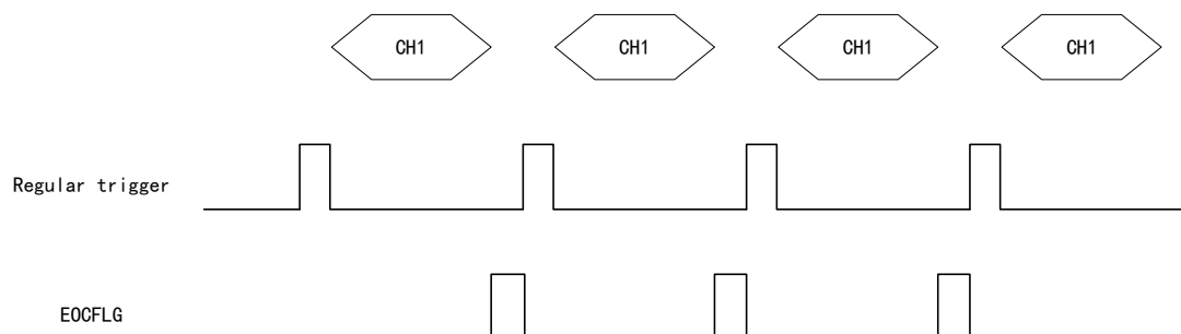
Figure 120 Single Conversion Mode Timing Diagram
