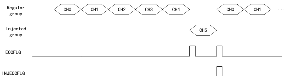
Figure 125 Automatic Injection Timing Diagram
