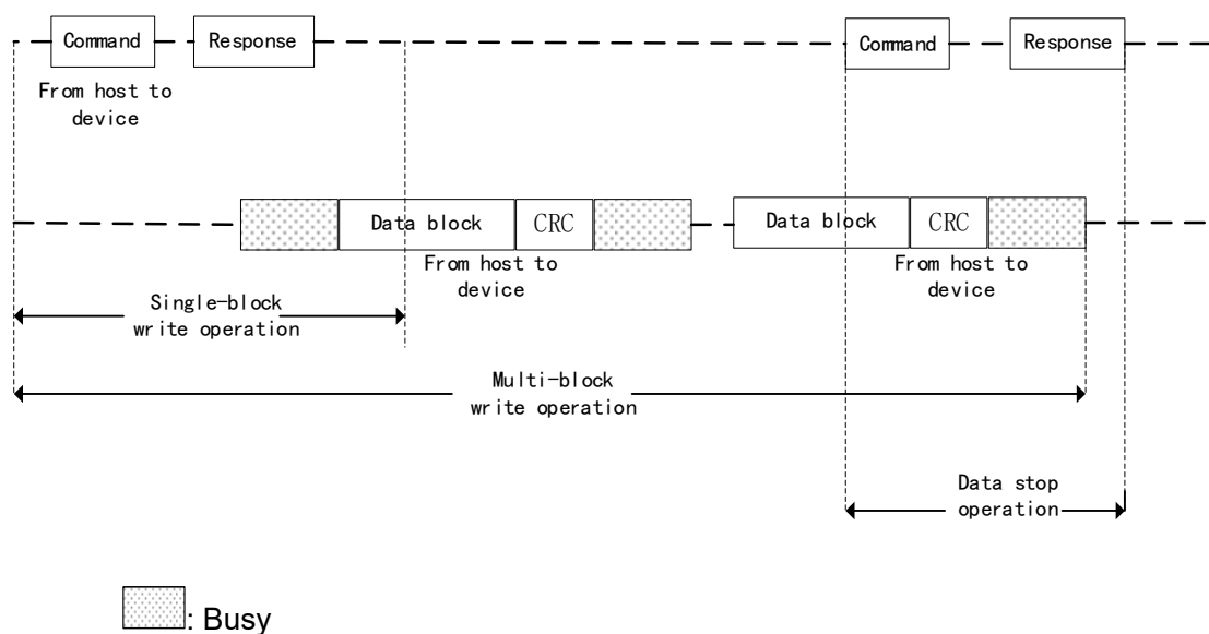
Figure 115 SDIO (Multi-) Data Block Write Operation
