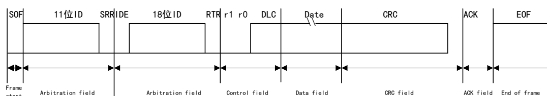
Figure 104 Extended Data Frame
