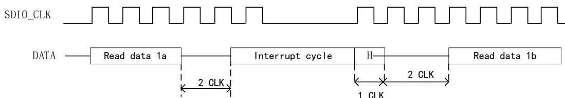
Figure 119 Read Wait Operation through Stop SDIO_CLK
