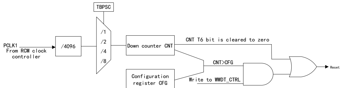
Figure 64 Window Watchdog Structure Block Diagram
