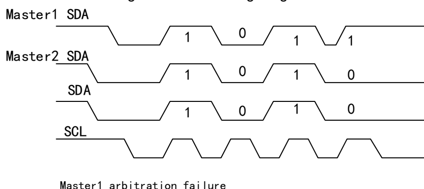
Figure 87 SDA Timing Diagram
