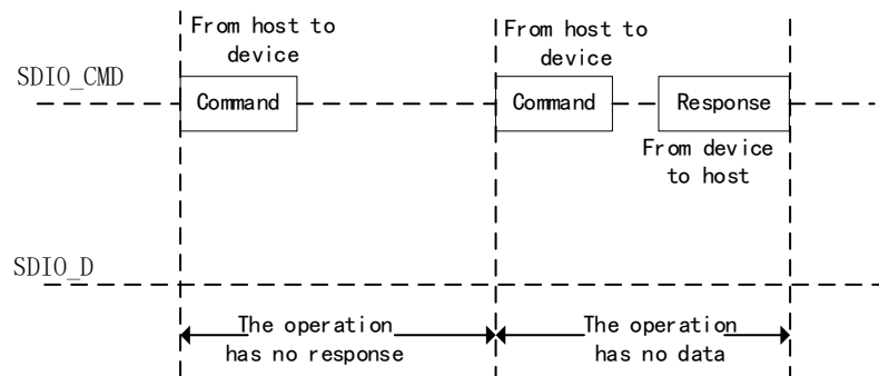
Figure 113 SDIO "No-response" and "No-data" Operation
