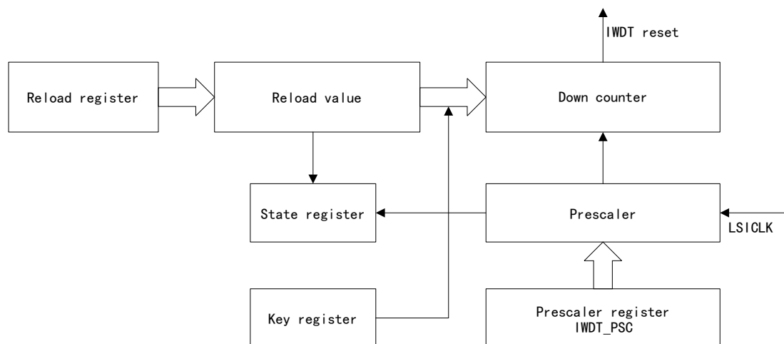
Figure 63 Independent Watchdog Structure Block Diagram
