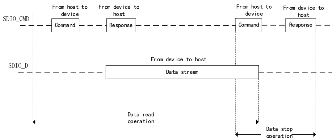
Figure 116 SDIO Data Flow Read Operation
