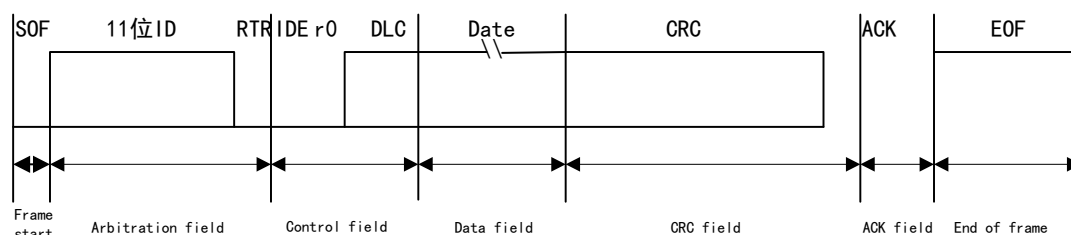
Figure 103 Standard Data Frame
