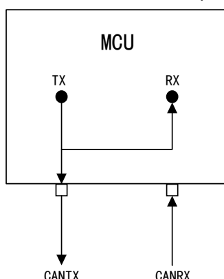
Figure 106 CAN Works in Loopback Mode
