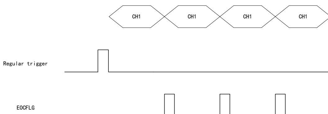
Figure 121 Continuous Conversion Mode Timing Diagram
