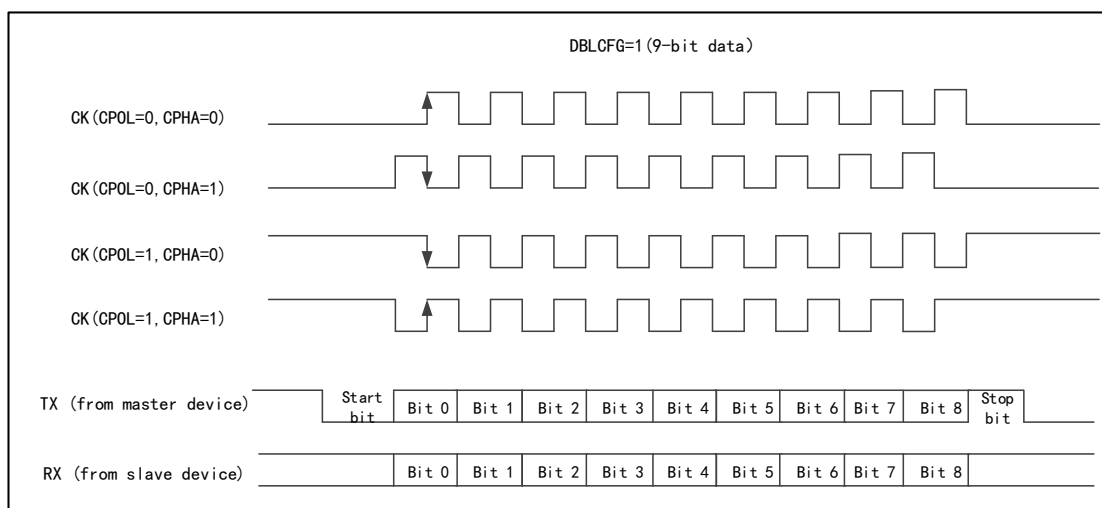
Figure 73 USART Synchronous Transmission Timing Diagram (DBLCFG=1)
