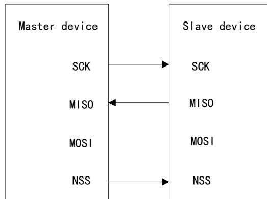
Figure 89 Connection in Half-duplex Mode (the master is used for receiving, while the slave is used for transmitting)
